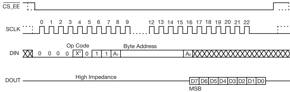
Figure 2-1. EEPROM Communications
